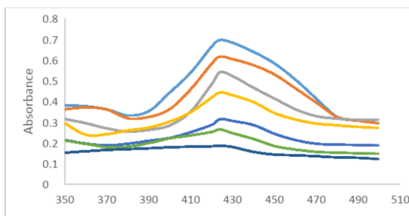
Figure 12: Photodegradation of Alizarin red
