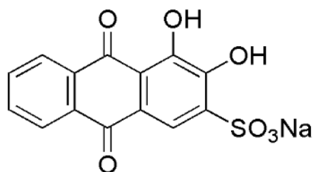
Figure 1: Chemical Structure of Alizarine red [10]
