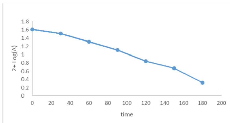
Figure 14: time vs 2+\log(A) graph of copper oxide nanoparticles
