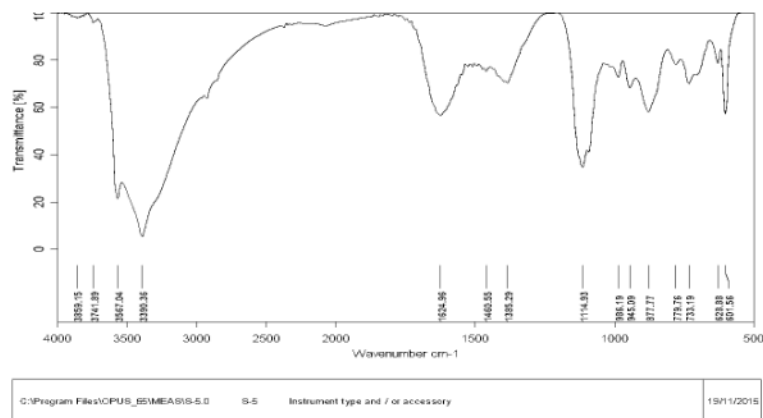
Figure 7: FTIR spectrum of copper oxide nanoparticles.
