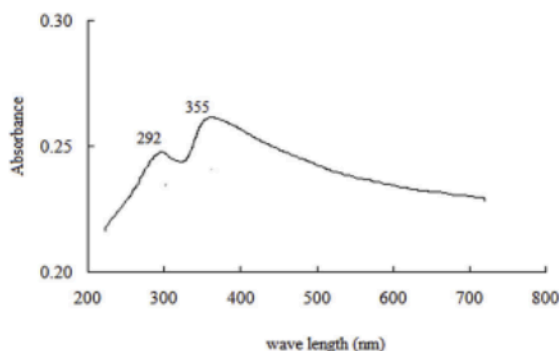
Figure 6: UV-Visible spectrum of copper oxide nanoparticles.
