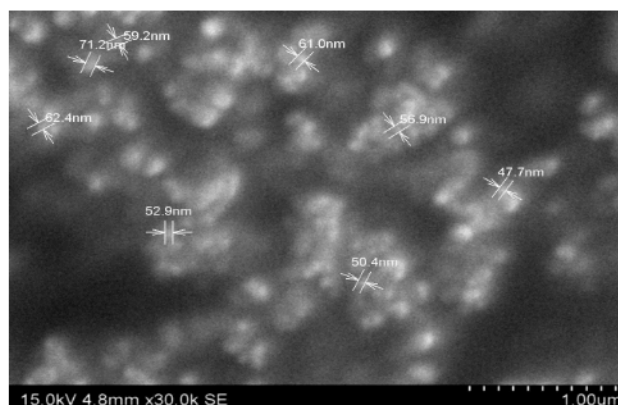
Figure 8: FESEM images of synthesized copper oxide nanoparticles.
